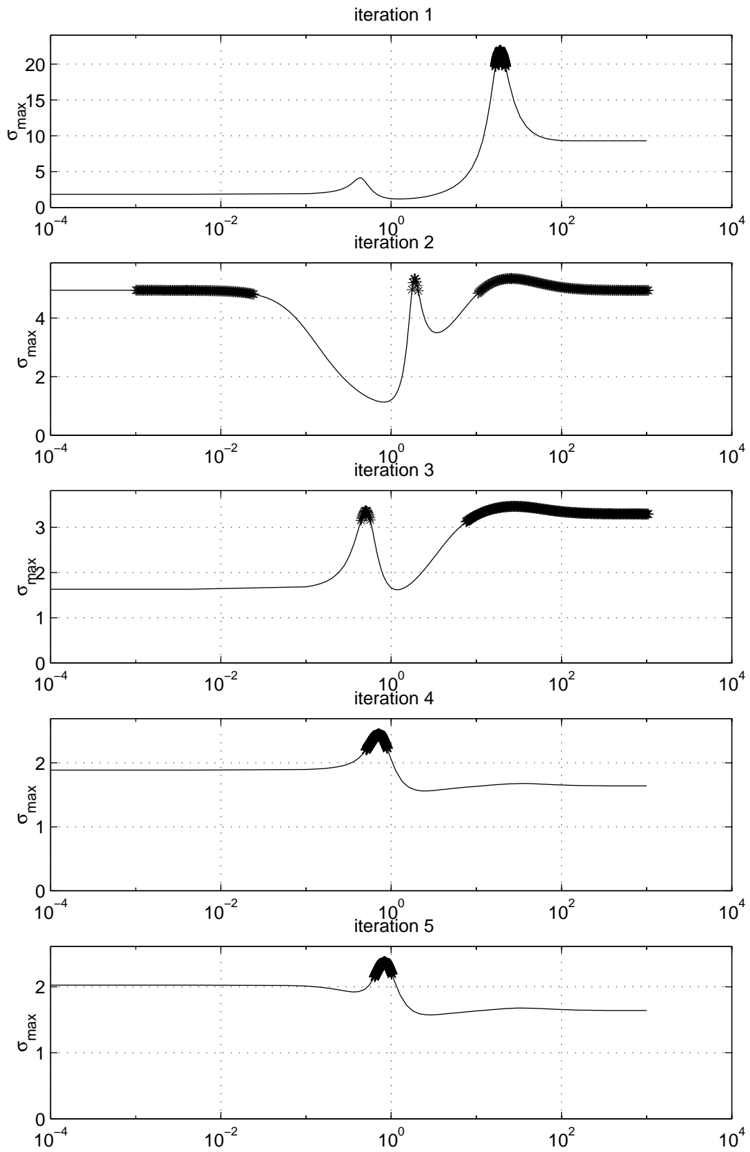
FIGURE 1: max singular values (transport airplane 'AC8') versus frequency first 5 iterations - '*' selected frequencies
