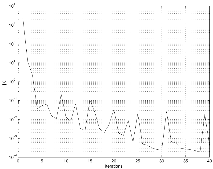
FIGURE 2: criticality measure \theta(x) versus iterations for 'BDT2'
